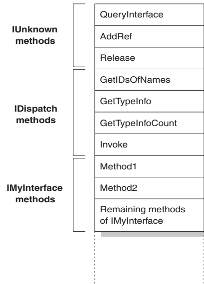
Figure 43.1 Dual interface VTable
